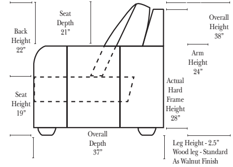
Rt-076 Arm Chair w/ 1/2 Curve
